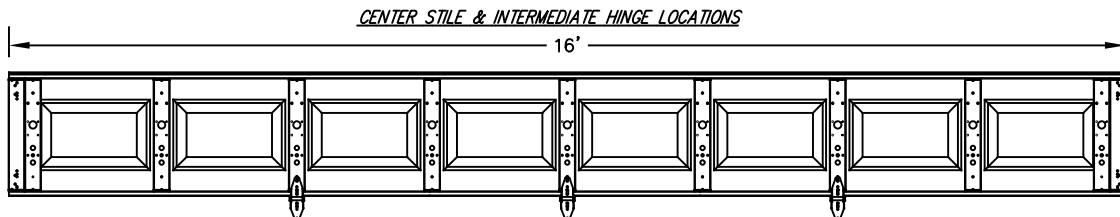
CENTER STILE & INTERMEDIATE HINGE LOCATIONS
